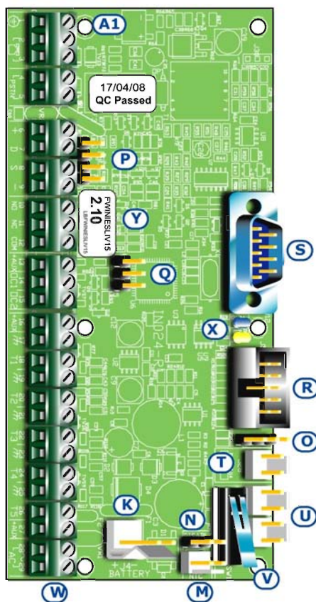
SmartLiving1050/1050L/10100L
