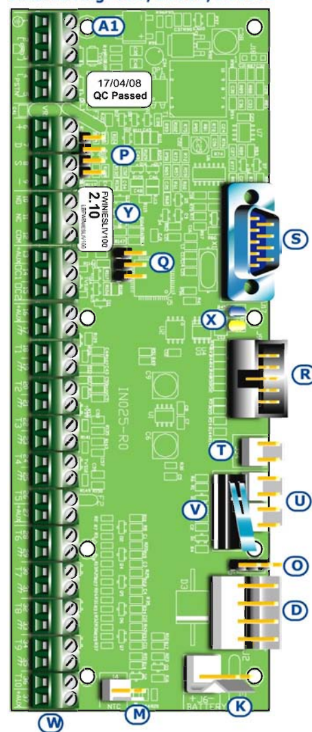
SmartLiving1050/1050L/10100L
