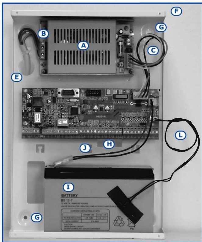
SmartLiving 1050
